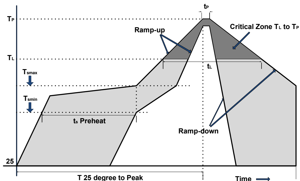
<Figure 6. Soldering Temperature time profile>
